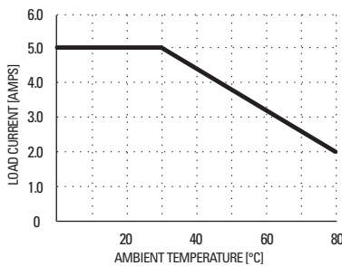
Max. Load Current vs. Temp.
